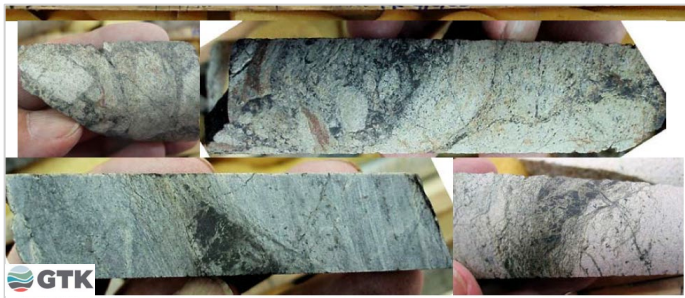
DH: R324 depth 42,55-42,90 m
